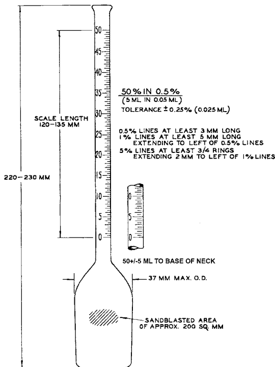
FIG. A1.1 Sulphonation Flask, Standard Babcock Bottle
