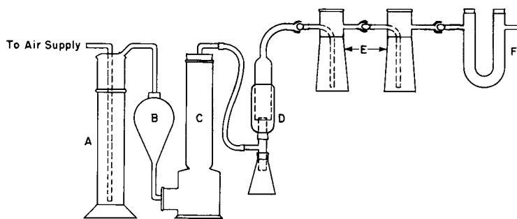
A—Sulfuric acid scrubber. B—Surge chamber. C—Drierite, phosphorus pentoxide tower. D—Lamp and chimney. E—Absorption bulbs. F—Drierite tube.
