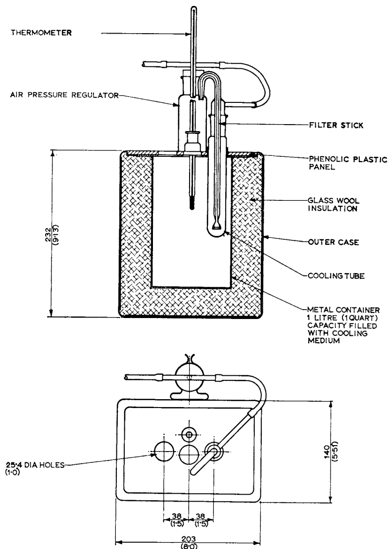
FIG. 2 Cooling Bath
