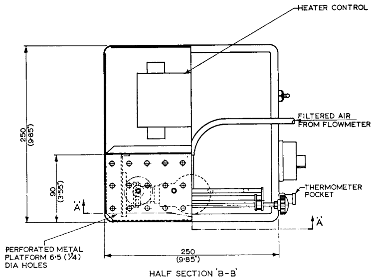
FIG. 4 Evaporation Assembly
