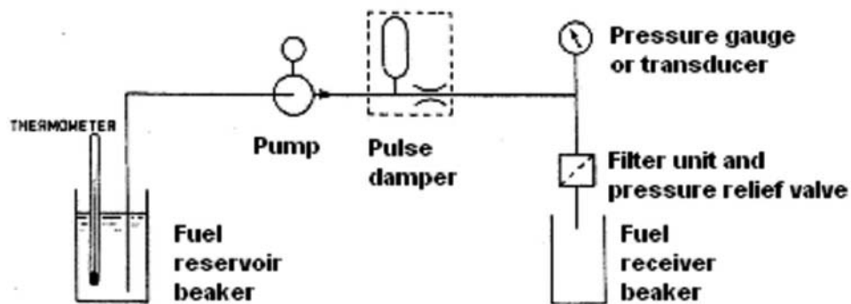
FIG. A1.1 Flow Diagram of Filtration Test Apparatus
