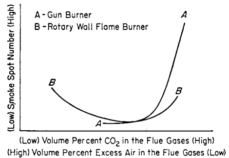
FIG. 1 Typical Smoke-CO 2 and Excess Air-CO 2 Curves
