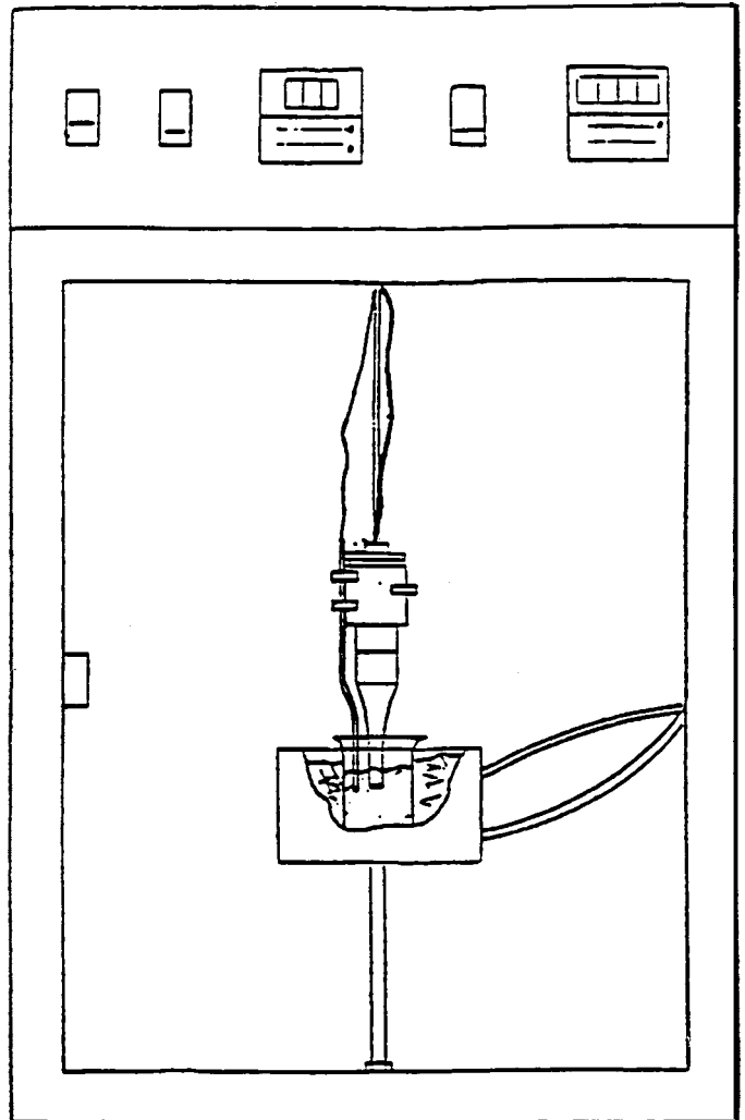
FIG. 1 Schematic of Sonic Probe Type Apparatus, Support Systems, Cabinet and Power Supply
