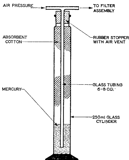
FIG. 3 Air Pressure Regulator
