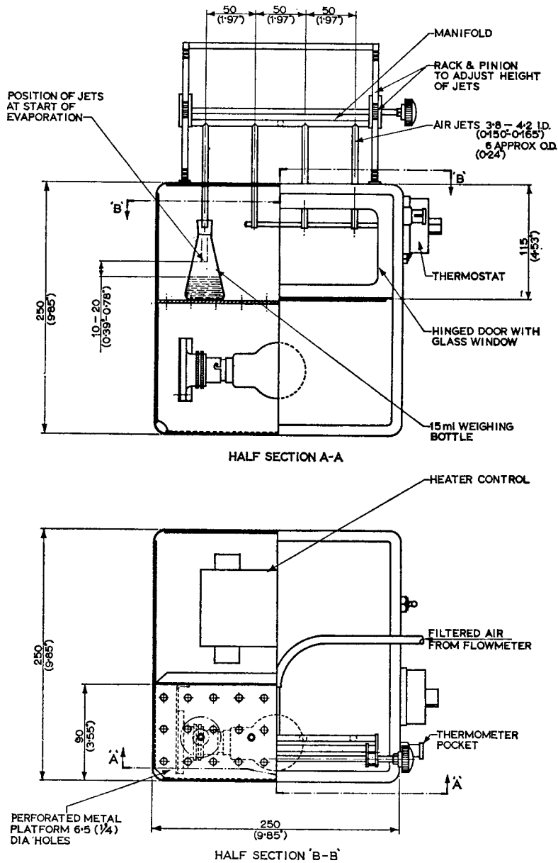
FIG. 4 Evaporation Assembly
