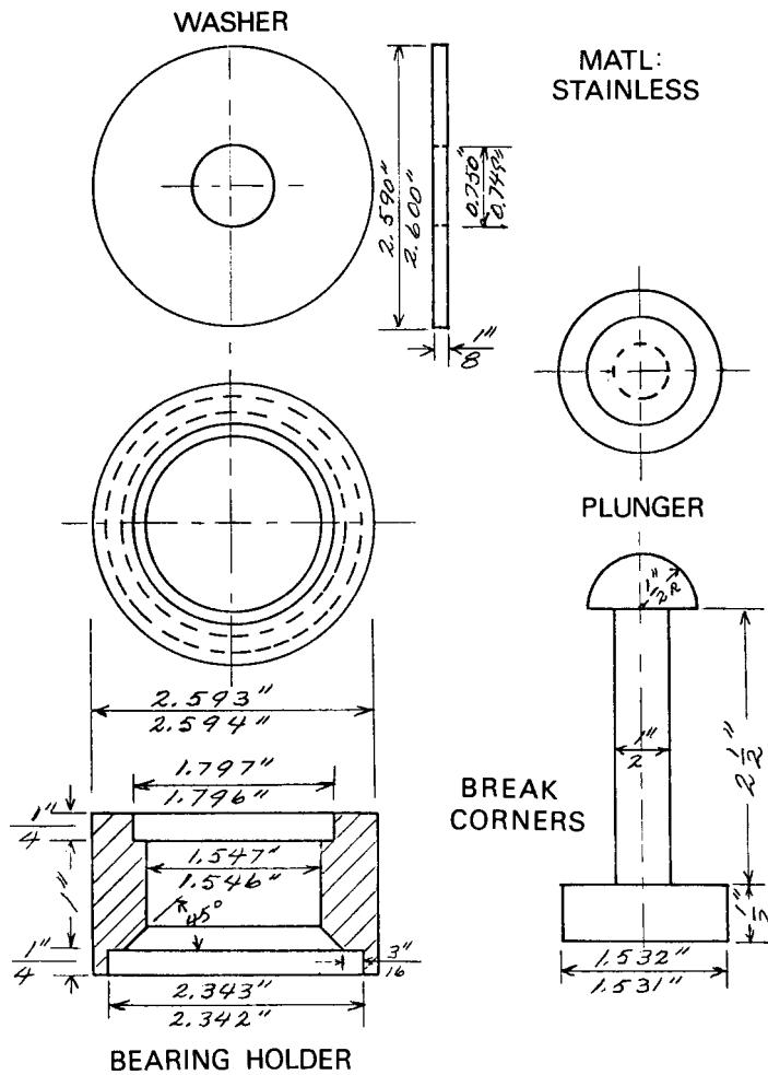
FIG. 6 Bearing Packer
