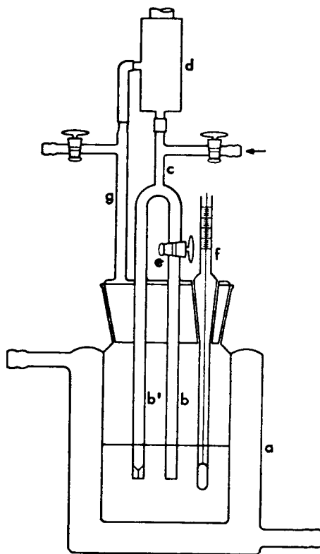
FIG. 1 Bubbler Unit
