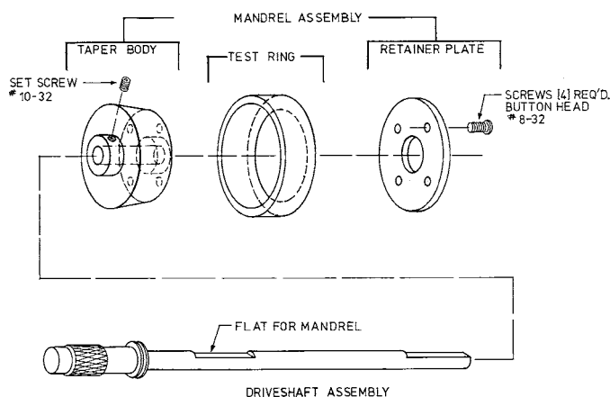
FIG. 2 Ring and Mandrel Assembly (Cylinder)
