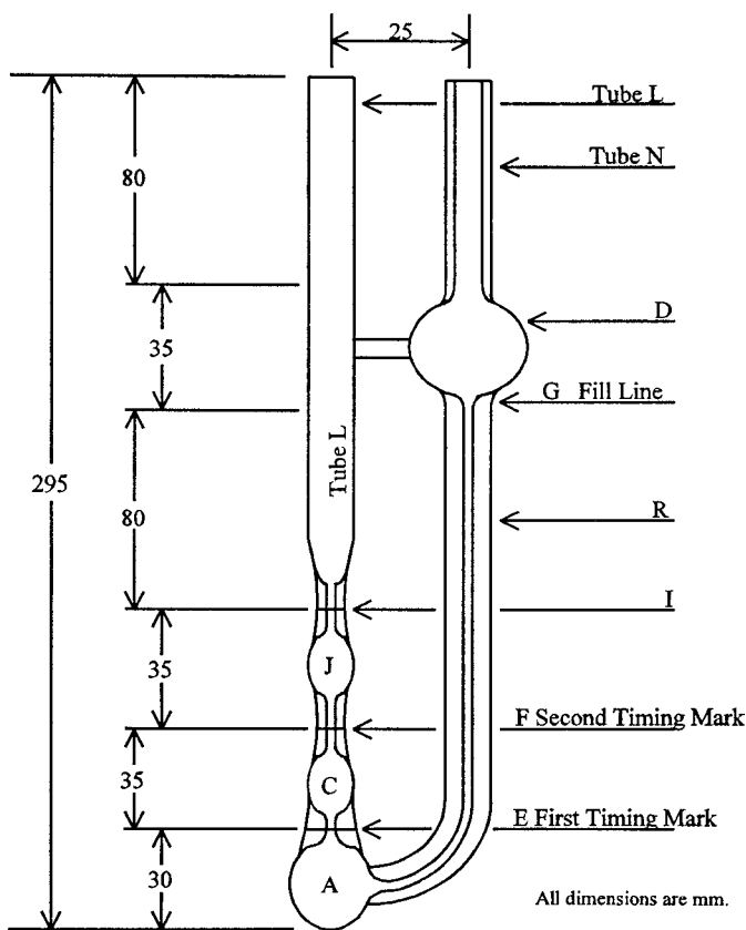
FIG. A3.2 Reverse Flow Viscometer
