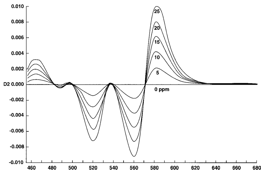
FIG. 2 Second Derivative Scans of Solvent Red 26 Dye in Kerosine
