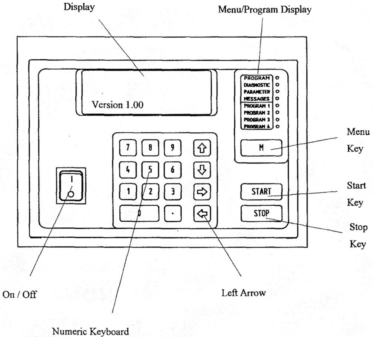
FIG. 4 Interface Panel
