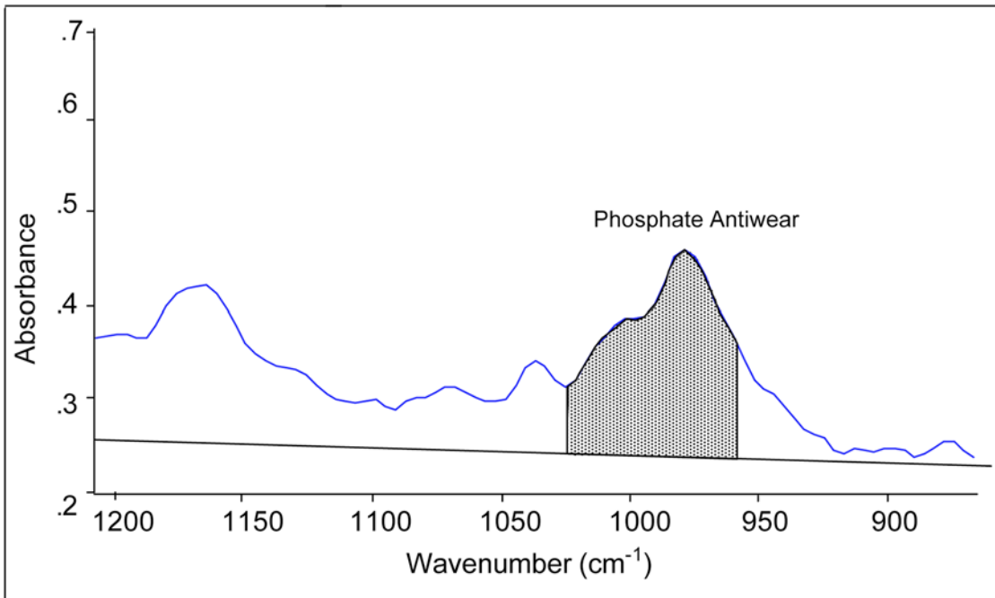
FIG. 1 Phosphate Antiwear Measurement in the Spectrum of a Diesel Crankcase Oil for Direct Trend Analysis (Procedure A)
