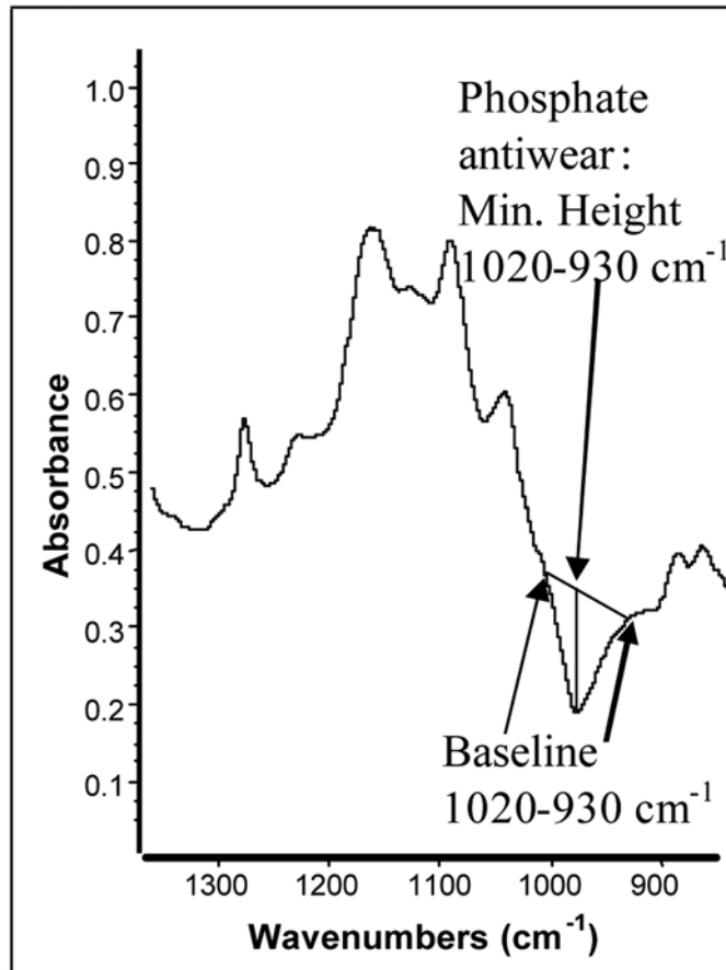
FIG. 2 Phosphate Antiwear Measurement in the Differential Spectrum of a Petroleum Crankcase Lubricant for Differential Trend Analysis (Procedure B)
