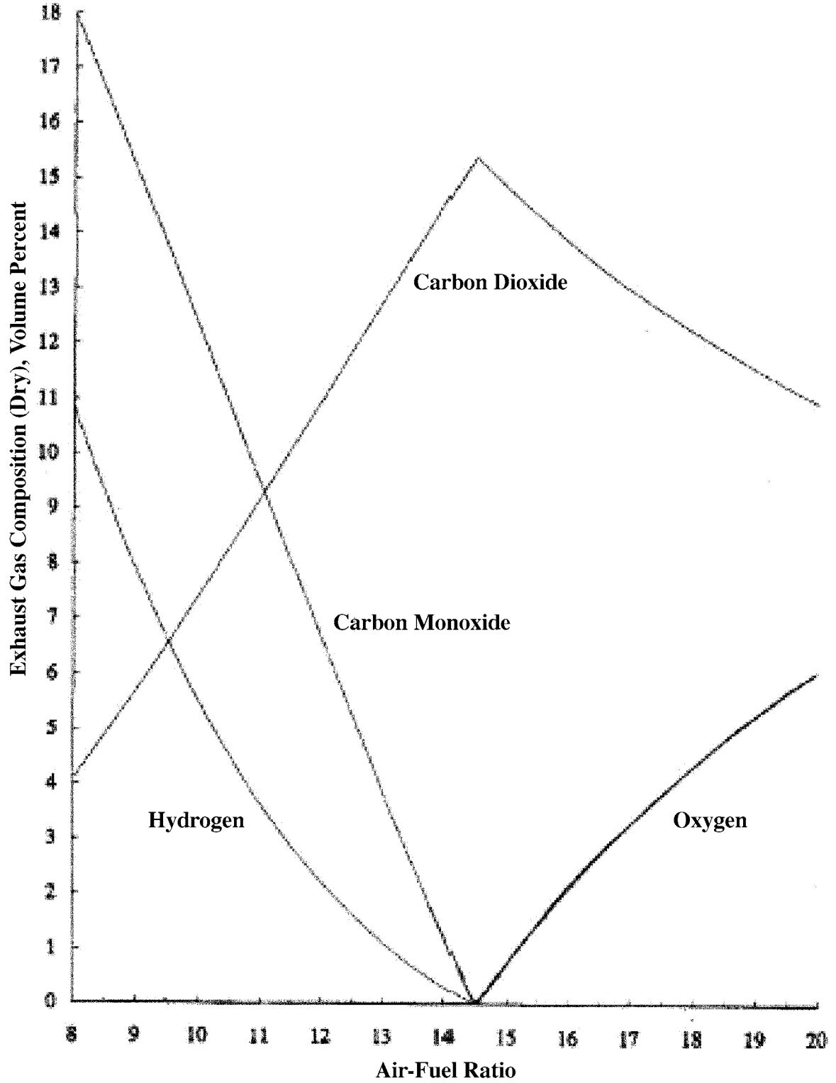
NOTE—Use corrected values for oxygen and carbon dioxide (see text). FIG. A6.2 Sequence IIIG Air-to-Fuel Ratio for Specified Fuel (C H 1.860 ) x
