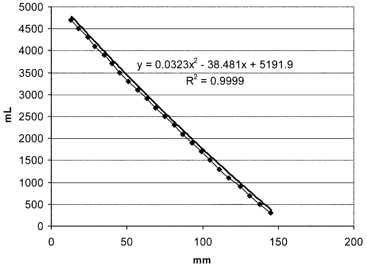
FIG. A3.1 Sequence III G Engine Oil Dipstick Calibration Curve
