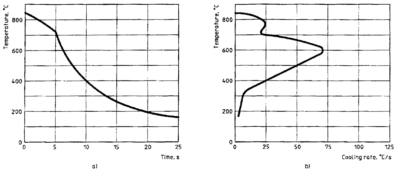
NOTE 1—(a.) Cooling Curve (b.) Cooling Rate Curve
