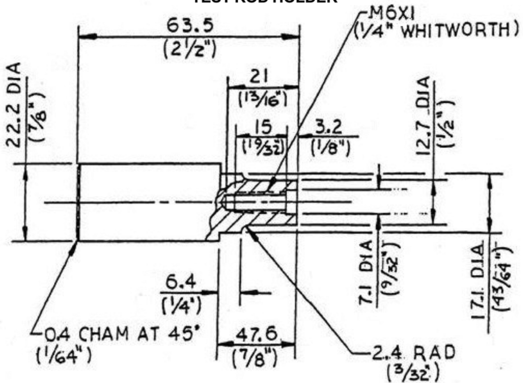
FIG. A1.3 Test Rod and Holder
