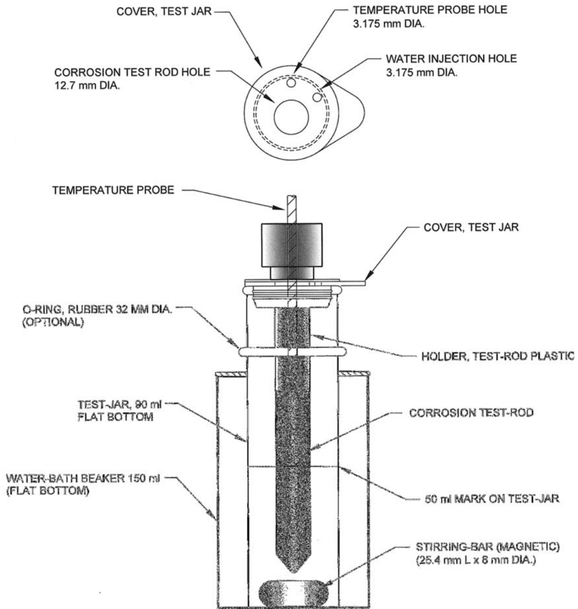
FIG. A1.1 Accelerated Iron Corrosion Test Apparatus
