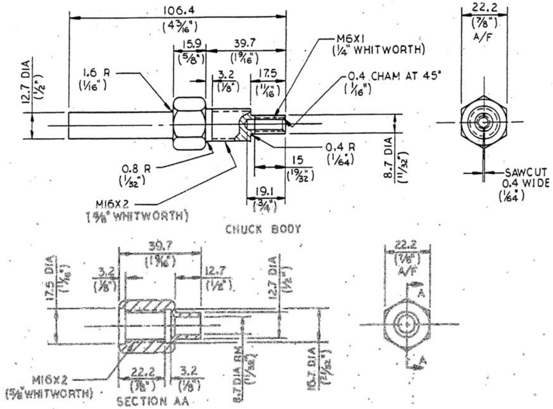
FIG. A1.4 Chuck for Polishing Test Rods
