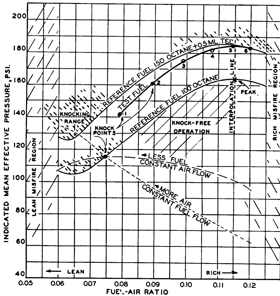
FIG. A2.4 Development of Knock-Limited Power Curves
