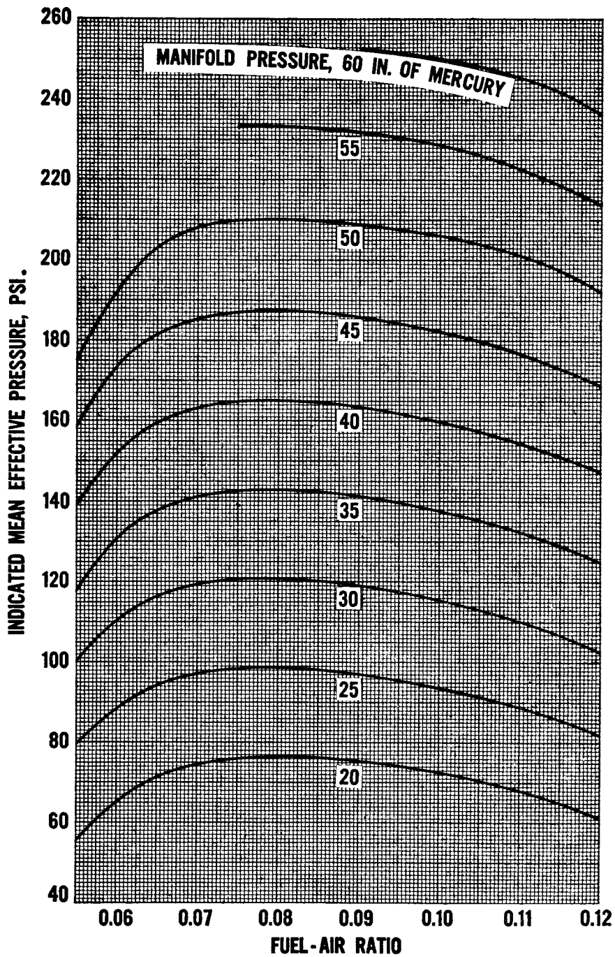
These Curves are for Isooctane plus 6.0 mL of Tetraethyllead per U.S. Gallon. FIG. A2.1 Average Power Curves at Several Constant Manifold Pressures
