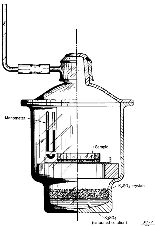
FIG. 1 Vacuum-Type Desiccator
