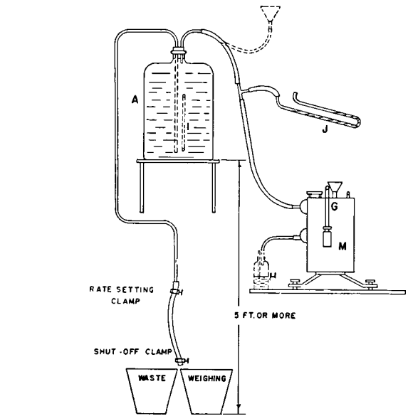
FIG. 6 Simple Equipment for Calibration by Aspirator Method
