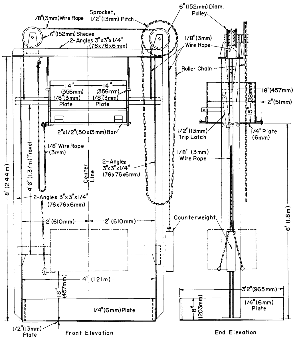
NOTE 1—1 in. = 25.4 mm FIG. 1 Shatter Test Machine
